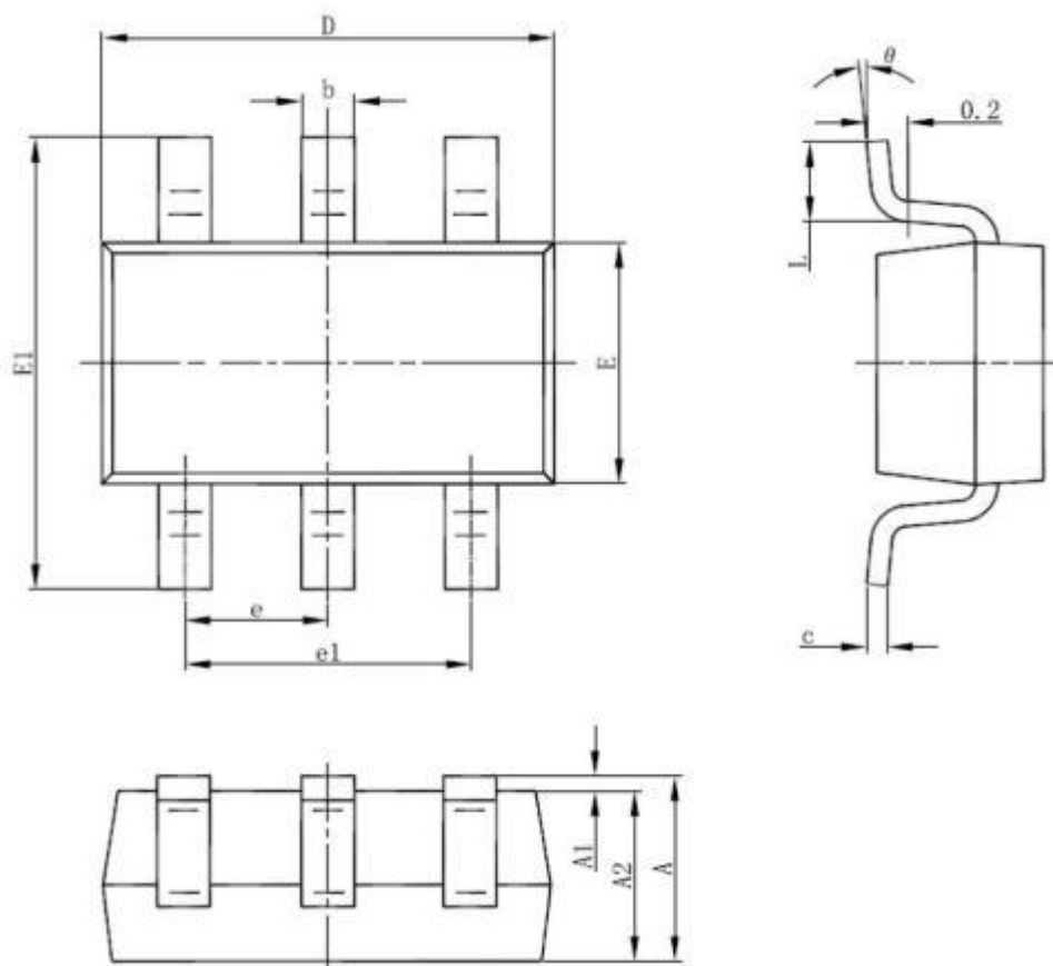
SOT23-6L (unit: mm)
